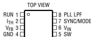
MS8 PACKAGE 8-LEAD PLASTIC MSOP T_{JMAX} = 125^{\circ}\text{C} , \theta_{JA} = 125^{\circ}\text{C/W}
